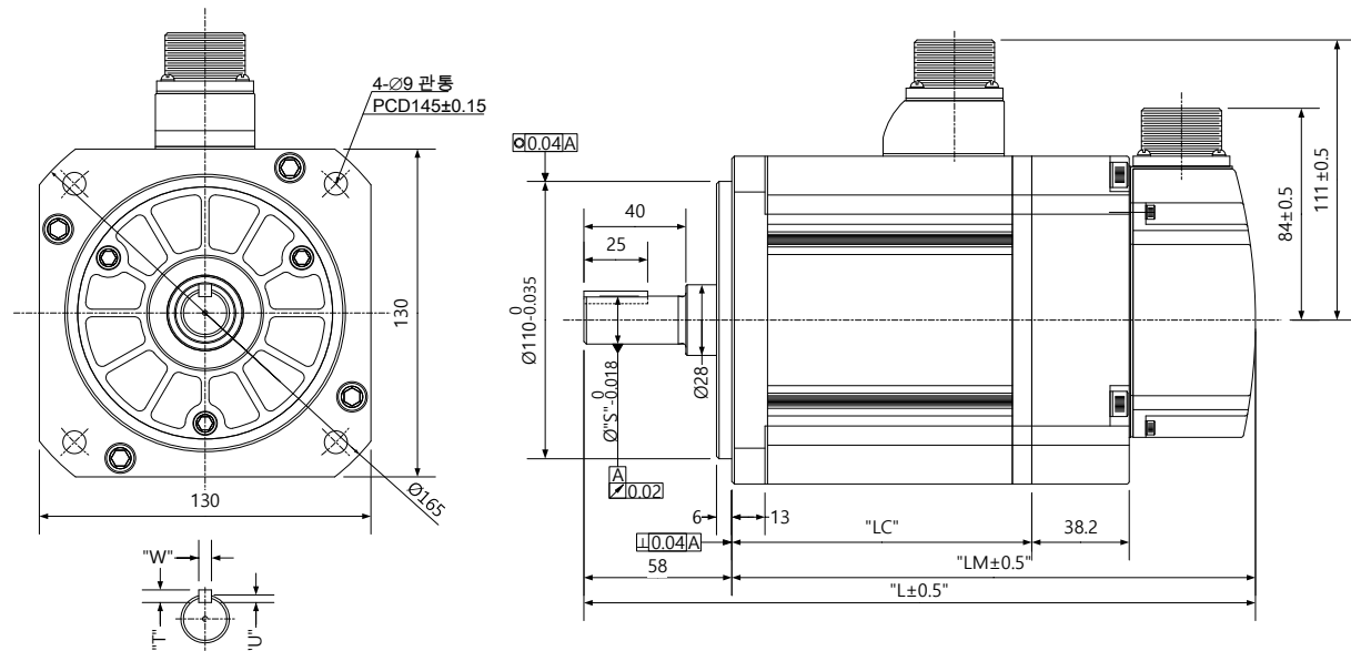
<Brake Type Connector>
