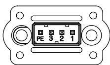
&lt;Power Connector 핀 배열&gt;
