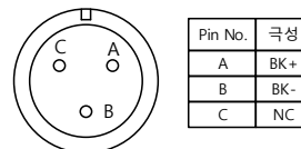
&lt;Brake Connector&gt;
