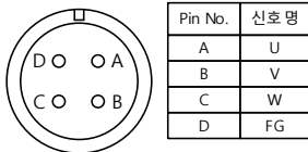
<Power Connector>
